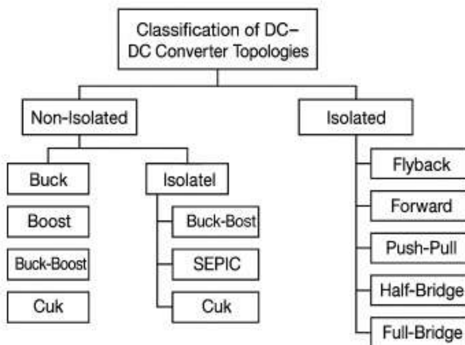
Figure 3.1 Classification of DC–DC Converter Topologies
