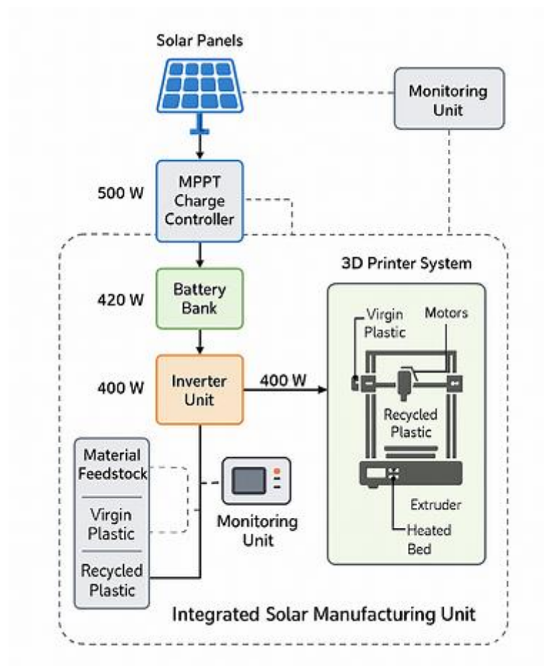
Figure 1: Conceptual Framework of Solar-Assisted Additive Manufacturing System
