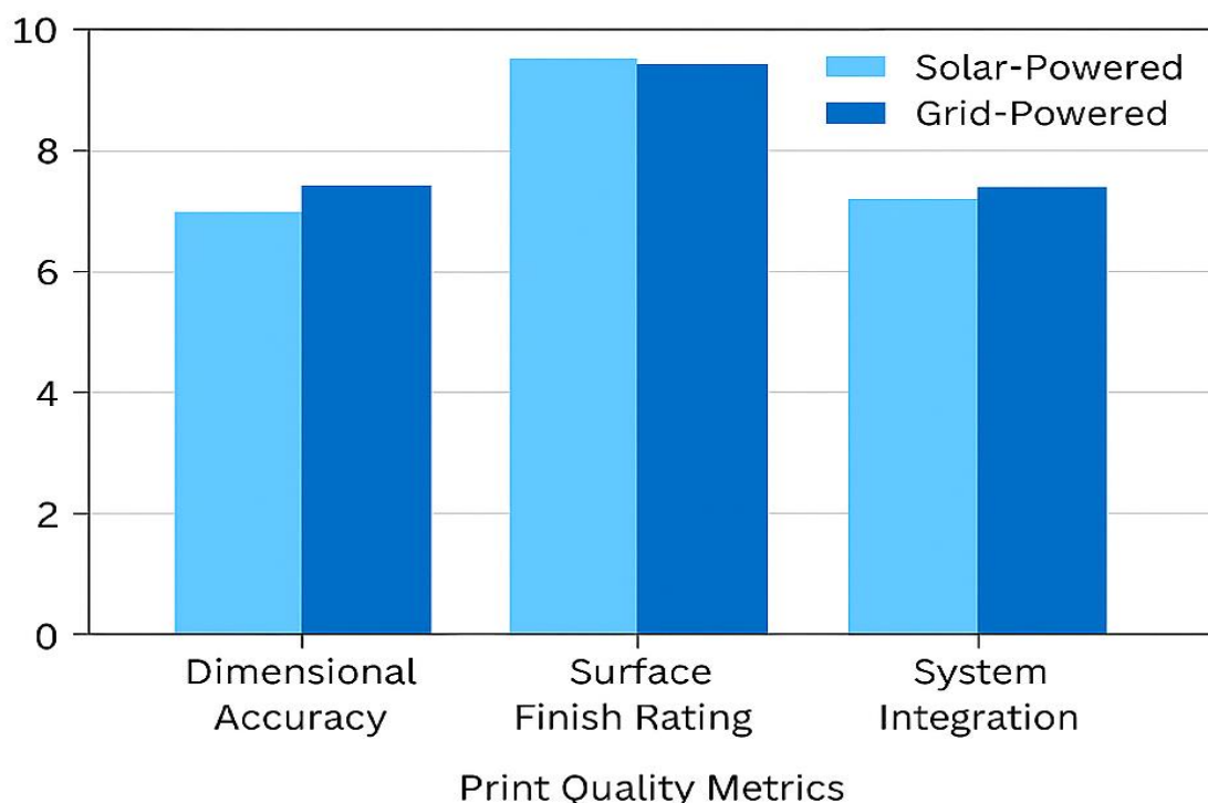
Figure 4: Print Quality Assessment of Solar-Powered 3D Printing System
