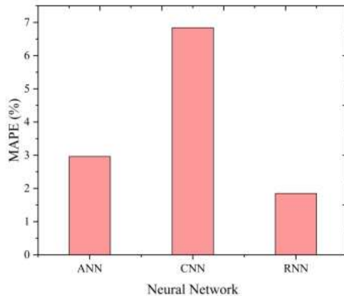
Fig 4 MAPE of neural networks
