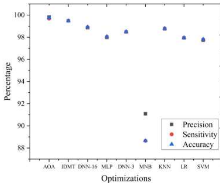
Fig 5 Precision, sensitivity, and accuracy of optimizer
