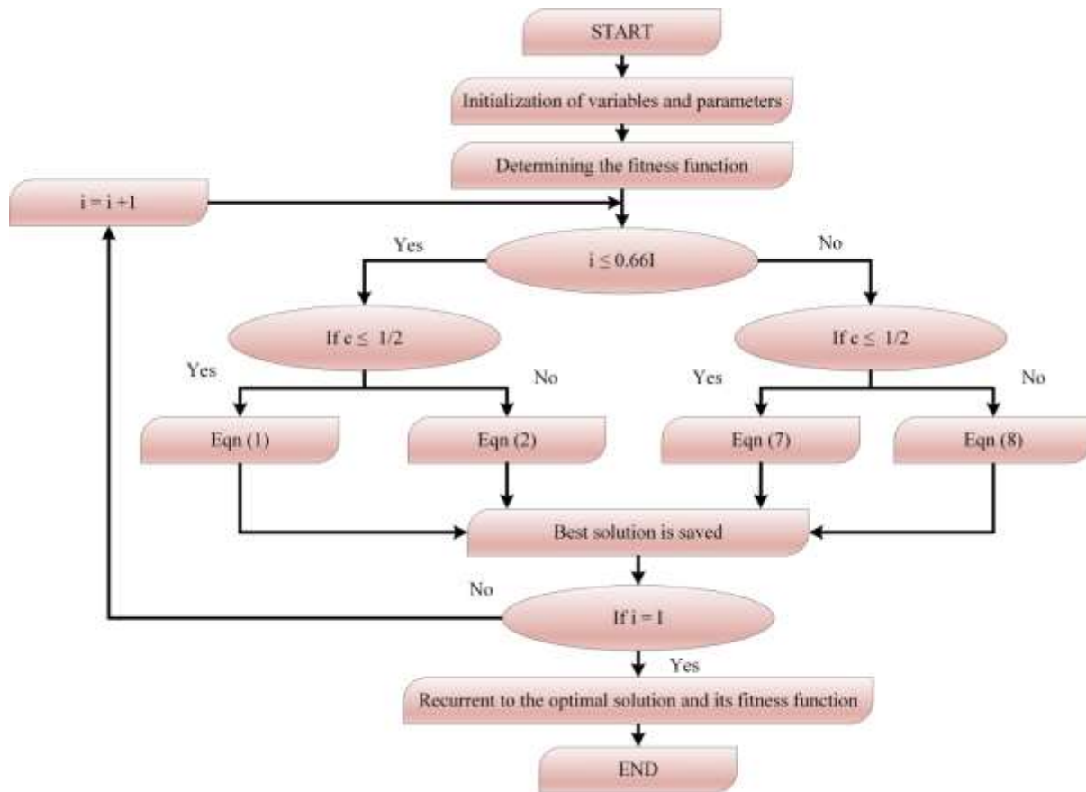
Fig 1 Flow diagram of AO
