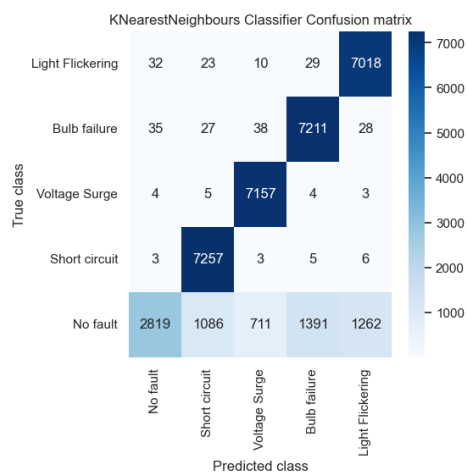
Fig 7: Confusion matrix of KNN Classifier model.
