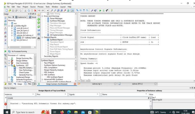
Figure 4: Delay estimation of the proposed system
