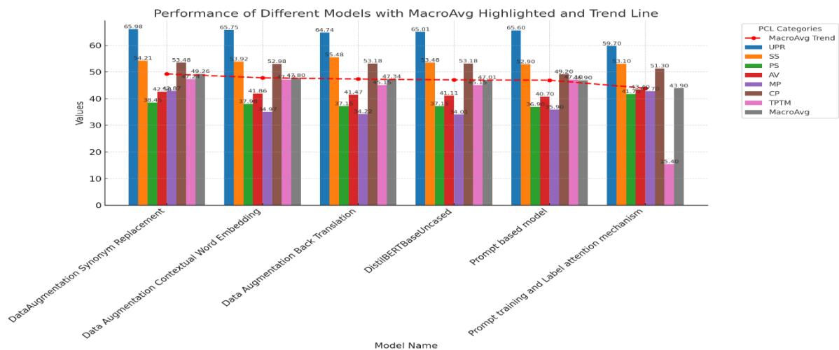
Figure 6: Macro F1 score of proposed and compared models
