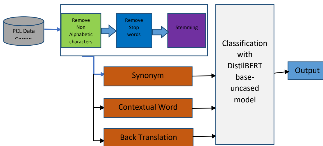
Figure 1: Proposed Model
