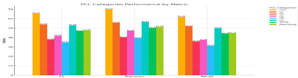
Figure 3: Metrics score of Fine-tuned DistilBERT with Data Augmentation Contextual Word Embedding
