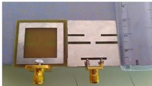
Figure 2. Fabricated antenna
