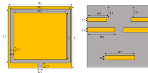
Figure 1. Antenna top view and rear view
