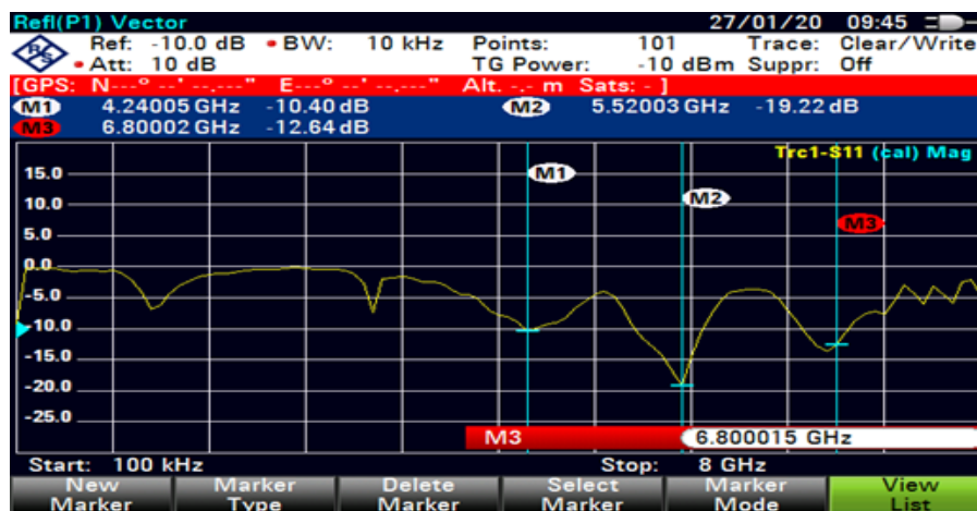
Figure 6. Experimental result using ZVH8 Vector network analyzer
