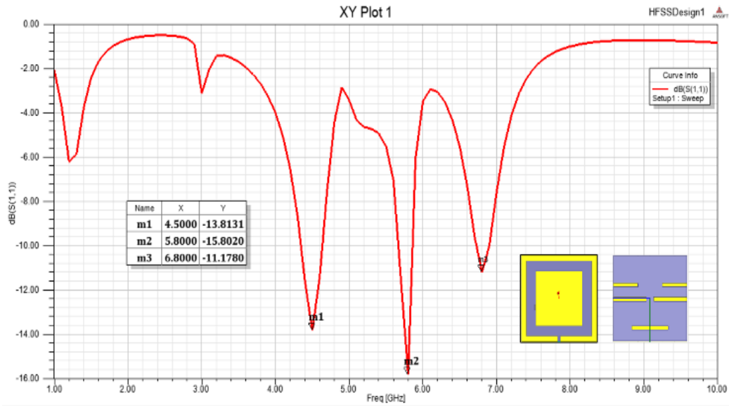
Figure 3. Return loss
